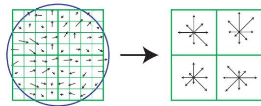
Fig. 1 SIFT descriptor generation. From left to right: Image gradients, and keypoint descriptor[5]
