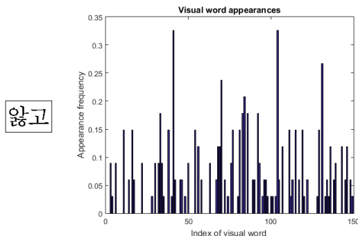
Fig. 5. Visual word vector. From left to right: original word block, and the visual word vector
