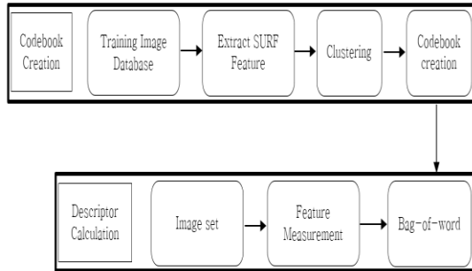
Fig. 4 Bag of Visual Word methodology
